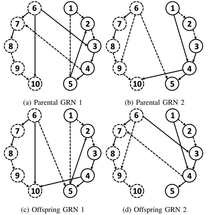
Fig. 5: Illustration of the diagonal recombination, with the pivot index as 5. Solid and dashed circles represent different modules. Solid and dashed arrows stand for activation and repression respectively.
